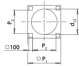
Foundation recesses 7)
