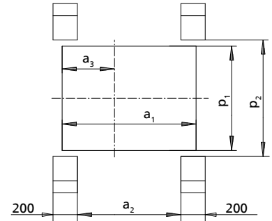
Foundation recesses 10)
