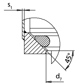
Detailed view Y: seating ring
