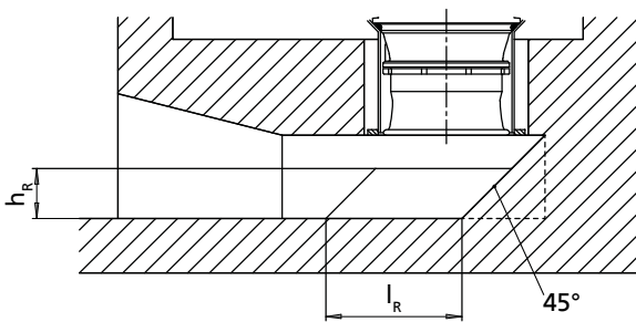
Fig. 2: Flow-straightening vane for covered intake chamber
