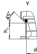
Detailed view Y: seat ring
