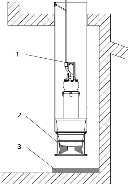
Fig. 1: Installation position of the pump set
