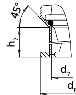
Detailed view Y: seat ring
