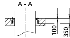
Foundation recesses 11)
