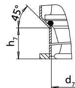
Detailed view Y: seat ring
