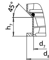
Detailed view Y: seat ring
