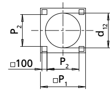
Foundation recesses 8)
