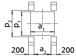
Foundation recesses 30)
