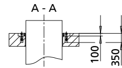
Foundation recesses 8)
