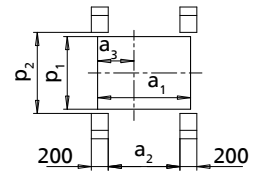
Foundation recesses 18)
