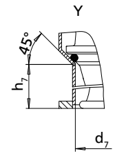
Detailed view Y: seat ring
