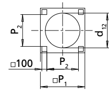
Foundation recesses 11)
